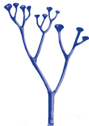
Cooksonia
